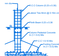
FOOTING DETAILS
