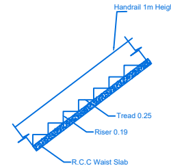
STAIR DETAILS
