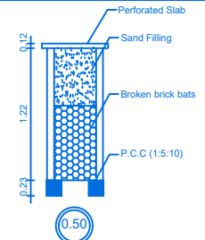
RAIN WATER COLLECTION WELL
