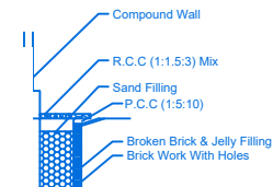
WATER HARVEST DETAILS
