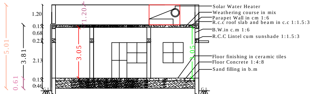
SECTION - "AB "
