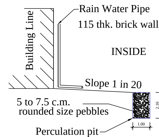
RAIN WATER HARVESTING PERCOLATION PIT
