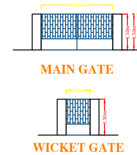
WICKET GATE
