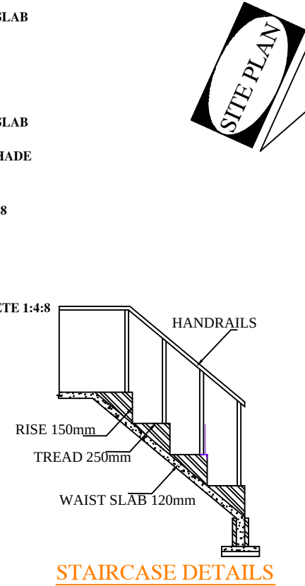
STAIRCASE DETAILS
