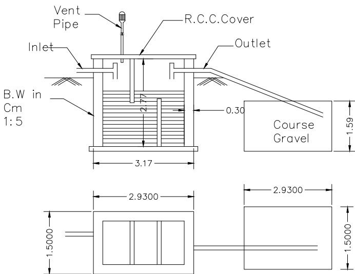
SEPTIC TANK & D-TRENCH DETAILS
