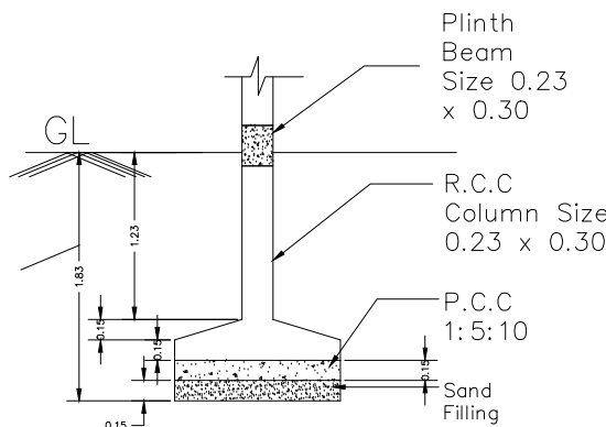
FOUNDATION DETAILS
