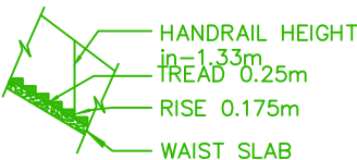
STAIRCASE DETAILS
