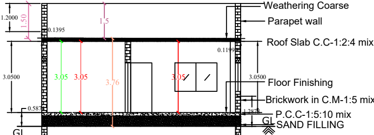
CROSS SECTION ON AB
