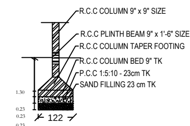
SECTION
