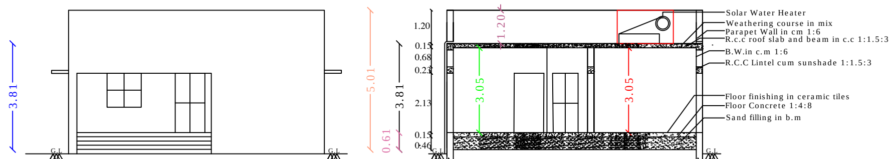
SECTION - "AB "
