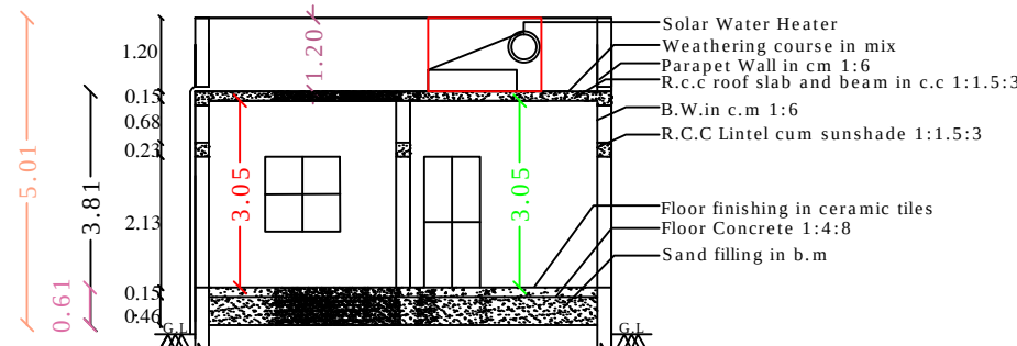
SECTION - "AB "
