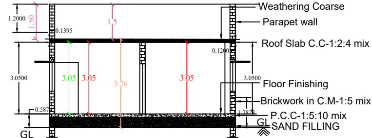
CROSS SECTION ON AB
