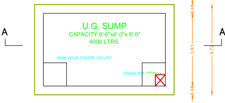
SUMP DETAIL SCALE 1"=4'0"
