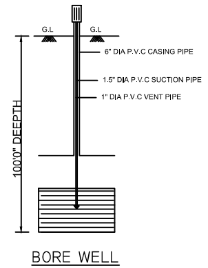
BORE WELL
