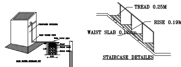
STAIRCASE DETAILS
