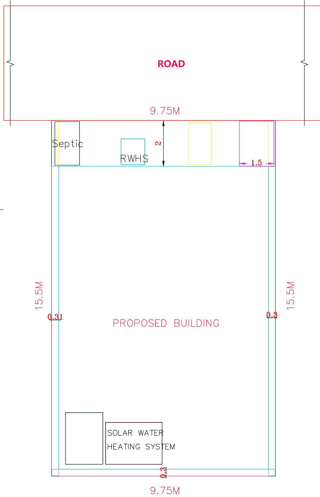
SITE PLAN
