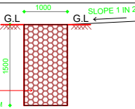
SECTION OF PEBBLE TRENCH SCALE : 1 : 100
