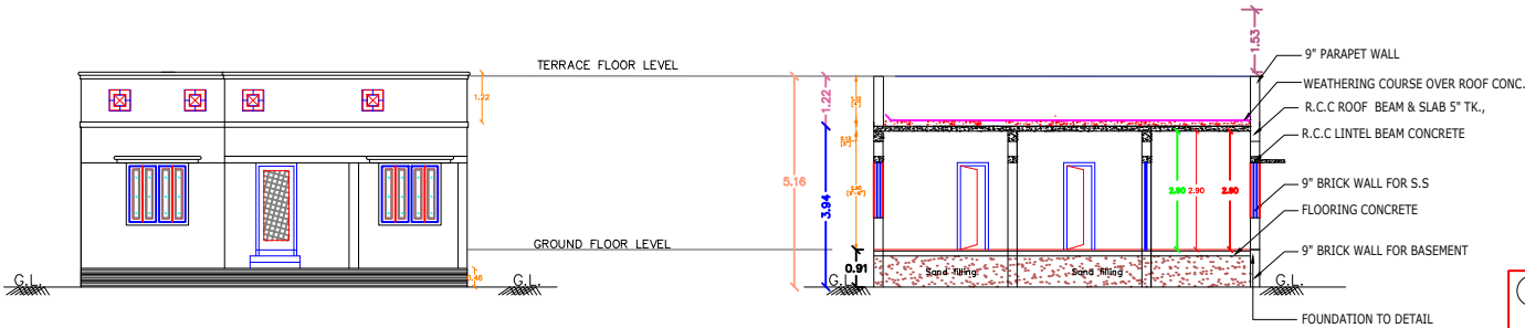
SECTION ON 'A-A'
