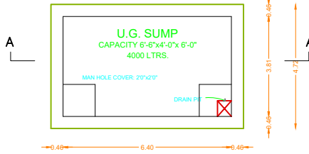
SUMP DETAIL
