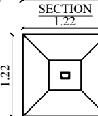
FOUNDATION DETAILS
