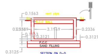
SECTION ON D-D
