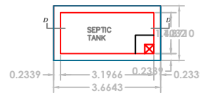
PLAN OF SEPTIC TANK
