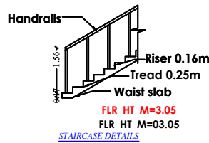
STAIRCASE DETAILS
