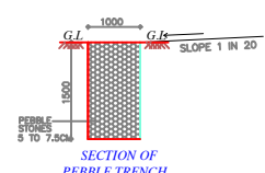
SECTION OF PEBBLE TRENCH
