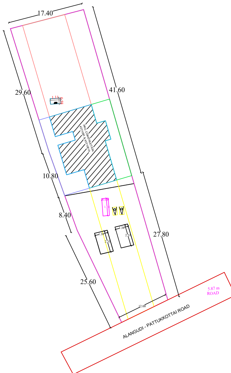
SOLAR SYSTEM
