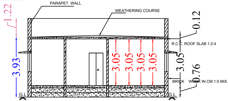
Section on-"AA"
