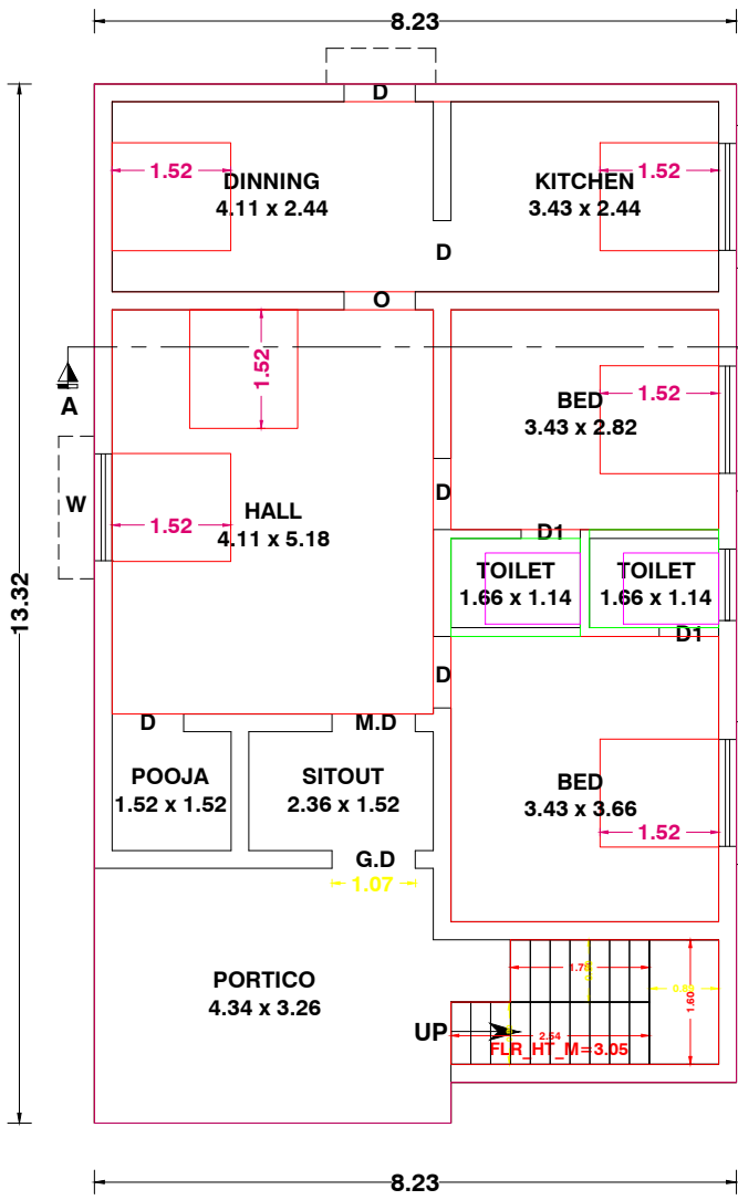
EXI.GROUND FLOOR PLAN
