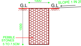
SECTION OF PEBBLE TRENCH SCALE : 1 : 100
