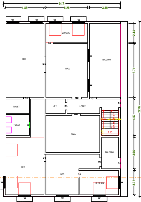
PROP.FIRST FLOOR PLAN
