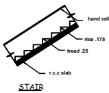
STAIR
