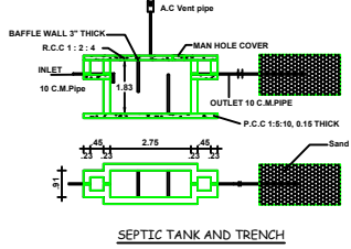
SEPTIC TANK AND TRENCH
