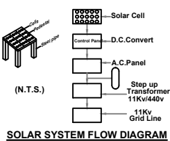
SOLAR SYSTEM FLOW DIAGRAM
