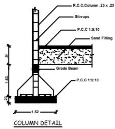
COLUMN DETAIL
