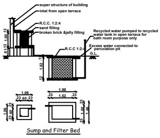
Sump and Filter Bed
