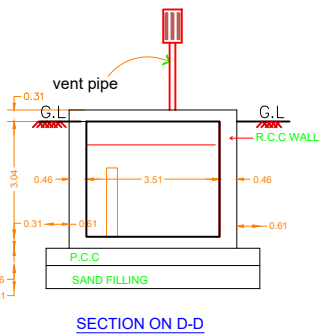
SECTION ON D-D
