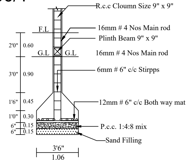
COLUMN DETAILS
