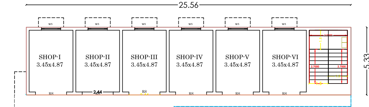
FLOOR PLAN
