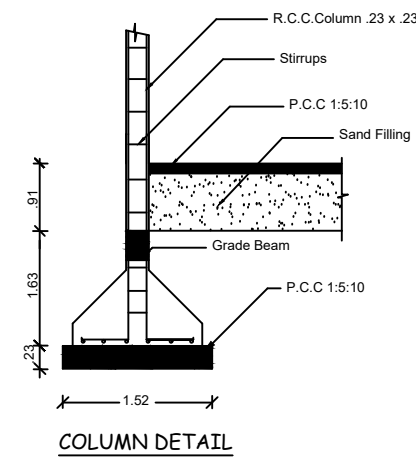
COLUMN DETAIL
