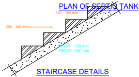
STAIRCASE DETAILS
