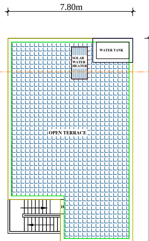
TERRACE PLAN
