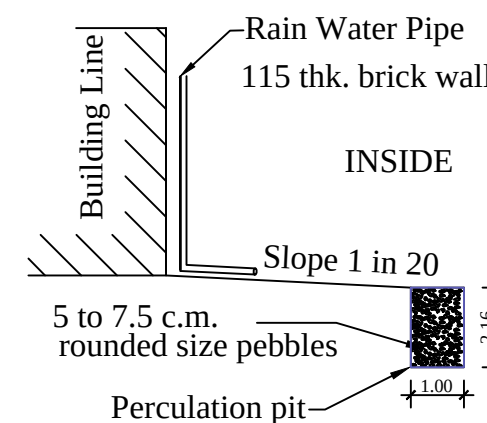
RAIN WATER HARVESTING PERCOLATION PIT RWH_CAPACITY_L=2000LTRS
