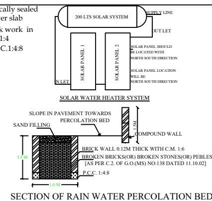
SECTION OF RAIN WATER PERCOLATION BED
