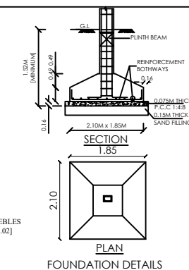
FOUNDATION DETAILS
