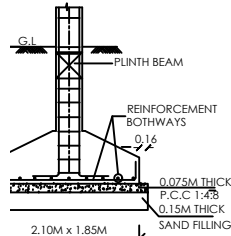
SECTION 1.85
