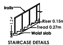
STAIRCASE DETAILS
