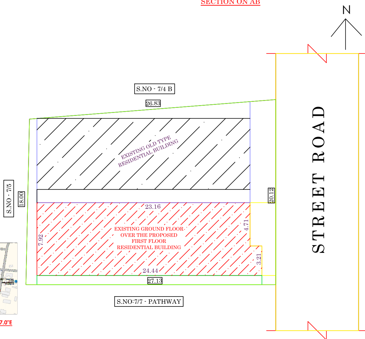
SITE PLAN
