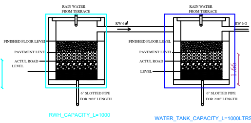
PLAN Compound wall Detail
