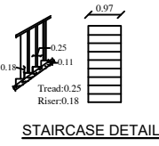
STAIRCASE DETAIL
