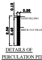
DETAILS OF PERCOLATION PIT
