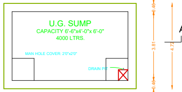
SUMP DETAIL SCALE 1"=4'0"
