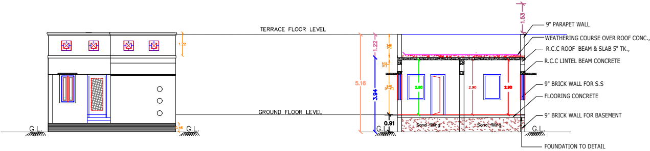
FRONT ELEVATION
