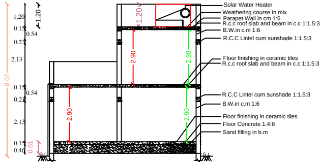
SECTION - "AB "
