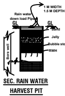
SEC. RAIN WATER HARVEST PIT
