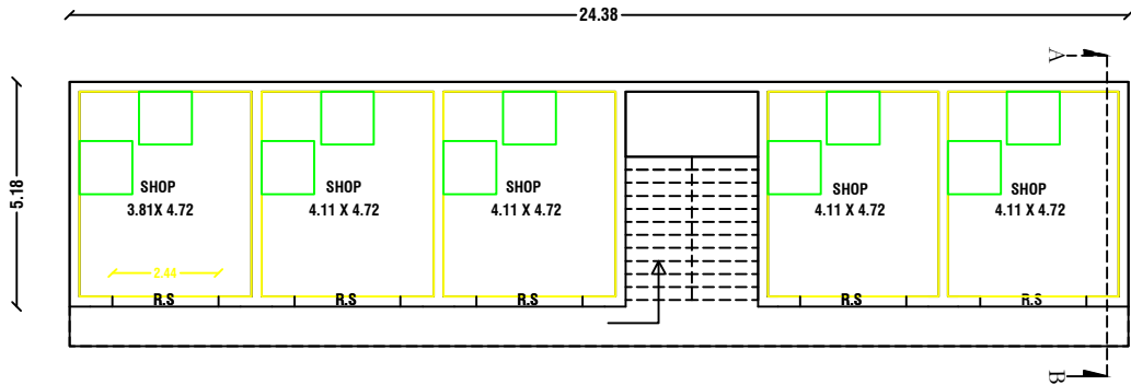
GROUND FLOOR
