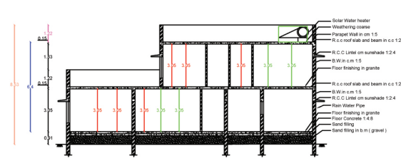
SECTION - "AB,CD"
