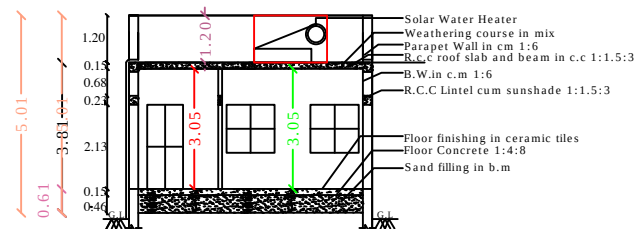
SECTION - "AB "
