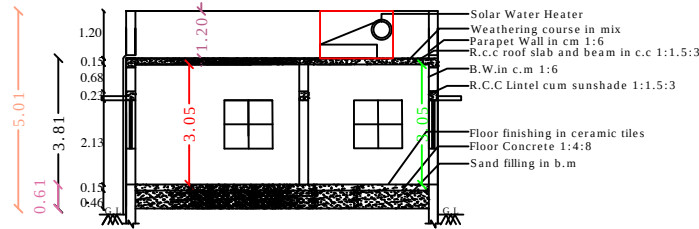
SECTION - "AB "
