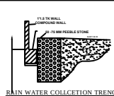
RAIN WATER COLLECTION TRENCH
