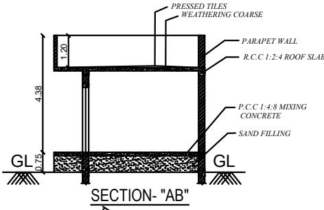
SECTION- "AB"
