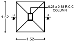
PLAN FOUNDATION DETAILS
