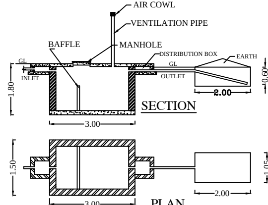
SEPTIC TANK DISPERSION TRENCH
