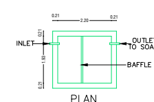
SEPTIC. TANK
