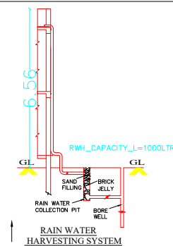
RAIN WATER HARVESTING SYSTEM
