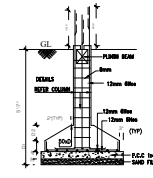
FOUNDATION DETAILS
