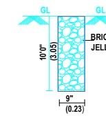
PERCULATION PIT
