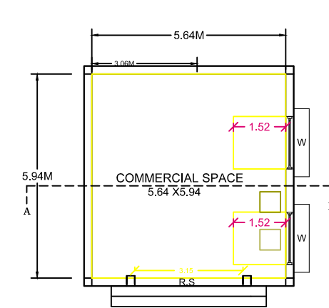
PRO. GROUND FLOOR
