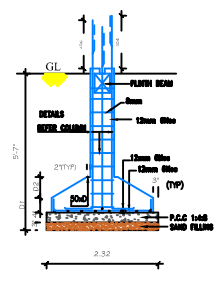
FOUNDATION DETAILS SCALE : 1:50.
