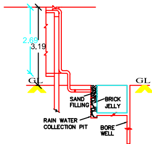
RAIN WATER HARVESTING SYSTEM RW_CAPACITY_L=1000LTRS
