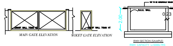
RWH SECTION (SAMPLE)
