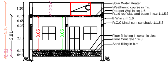
SECTION - "AB "
