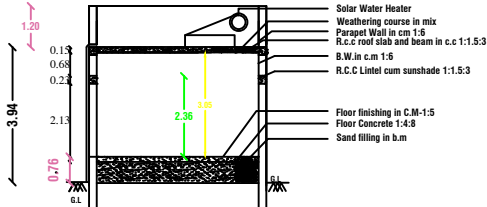
SECTION - "AB "
