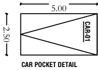
CAR POCKET DETAIL
