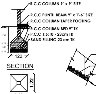
COLUMN DETAILS PLAN
