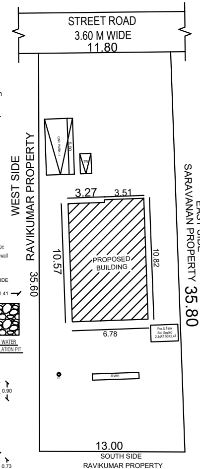
SITE PLAN SCALE 1:200
