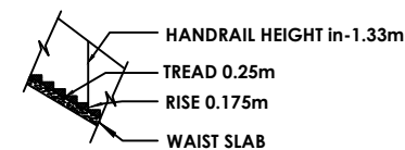
STAIRCASE DETAILS
