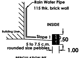
PERCOLATION PIT
