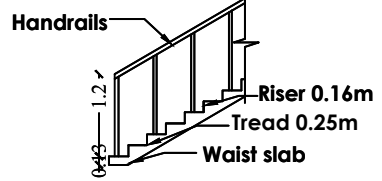
STAIRCASE DETAILS
