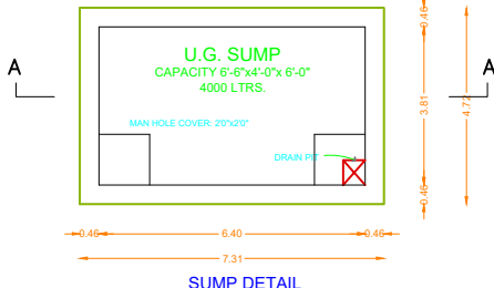
SUMP DETAIL SCALE 1"=4'0"
