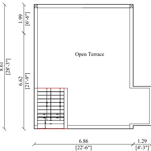
FURST FLOOR PLAN
