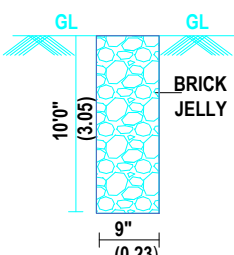
PERCULATION PIT
