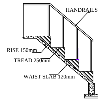
STAIRCASE DETAILS
