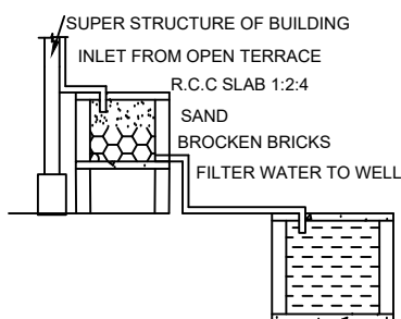
RAINWATER HARVESTING
