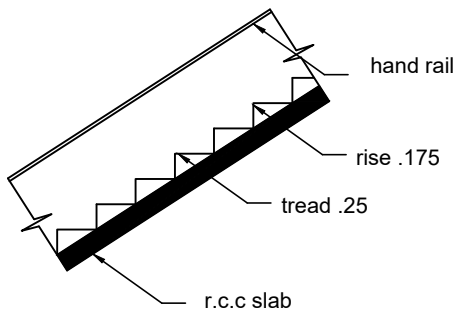
STAIR
