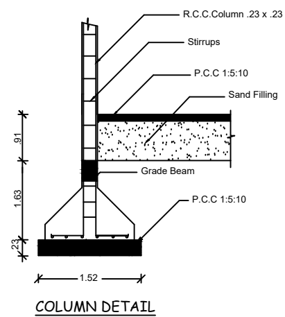
COLUMN DETAIL
